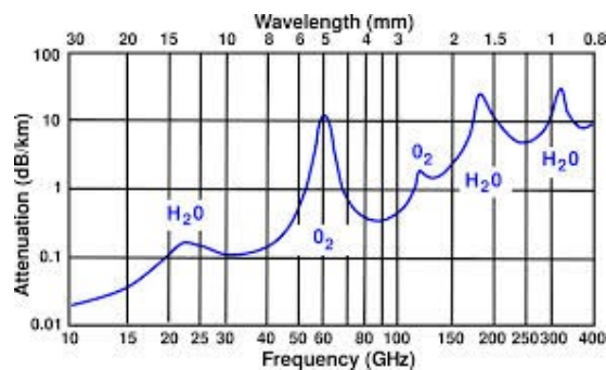
Figure 1: Atmospheric attenuation under different frequency bands
